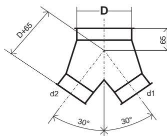
Hosenrohr 30° Culotte 30°
